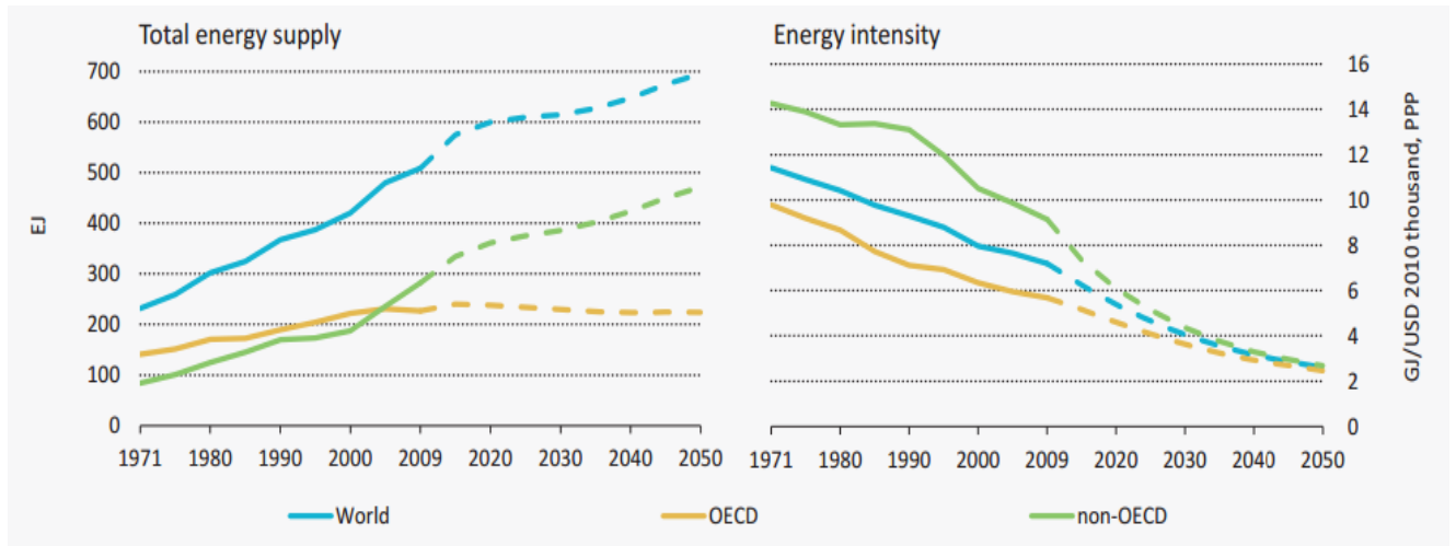
Fig. 2. Trends of the energy supply and energy intensity per unit of GDP under the 2DS scenario [1]
