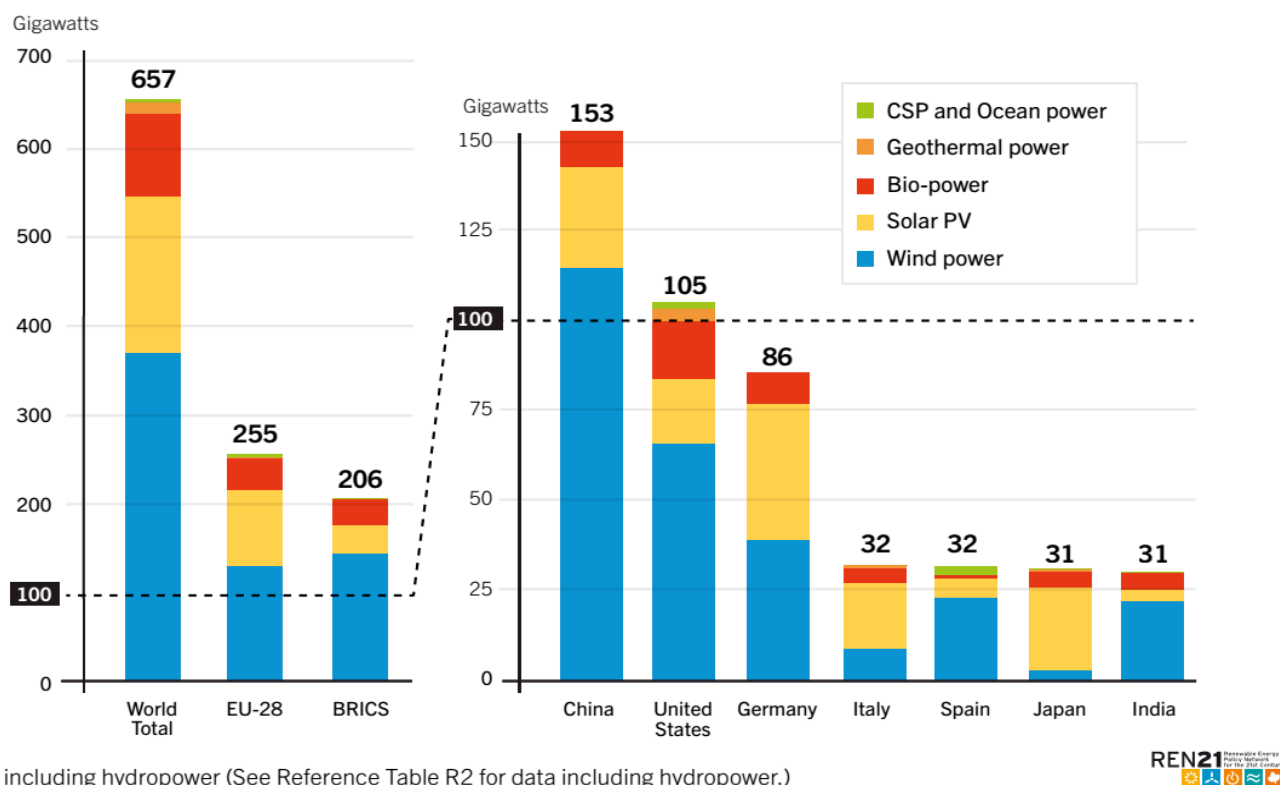
Fig. 6. Installed renewable electric capacity in the world 1 , 2014 [5]
