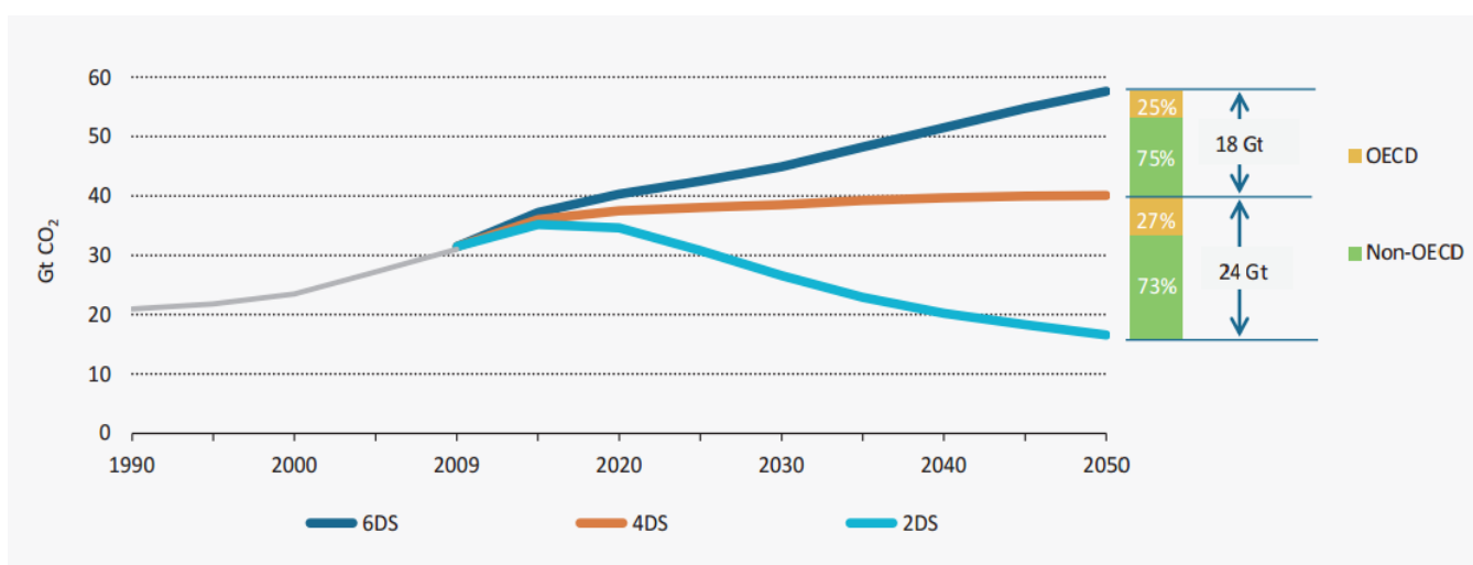
Fig. 1. Growth of GHG emissions in the world and climate change scenarios [1]
