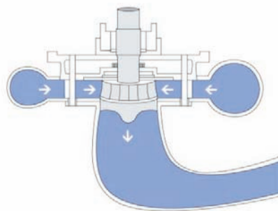
Francis turbine 5
