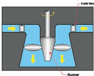
Propeller turbine 4
