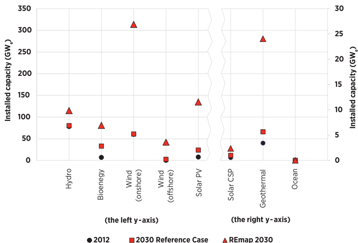
Figure 23: Power capacity by renewable energy technology
