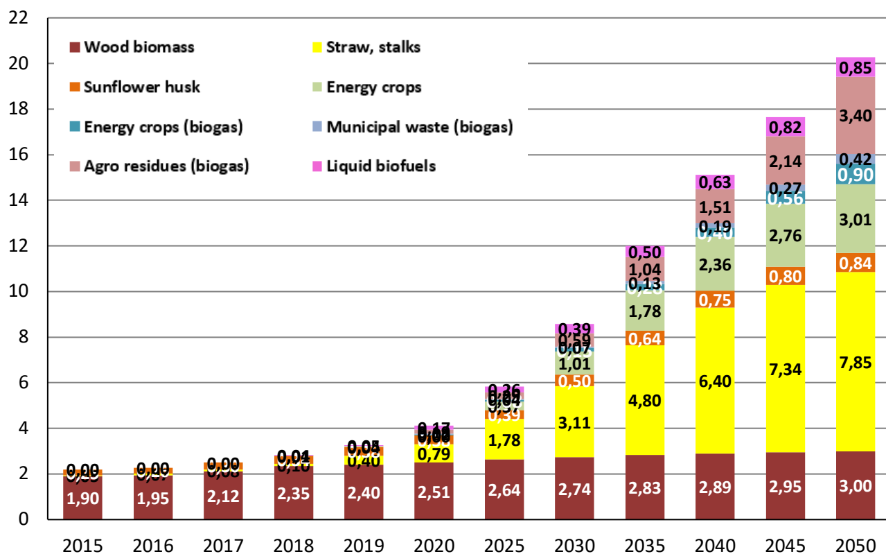
Fig. 5.17. Suggested structure of using biofuels in Ukraine until 2050, by type, Mtoe
