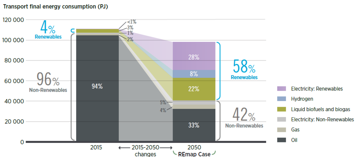
Fig. 5.11. Structure of the global transport final energy consumption until 2050 42
